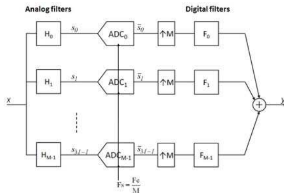
Figure 1. HFB architecture
