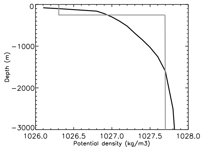
Figure 5. Potential density profile in the region east of the KP [from Park et al., 1993]. The two-layer approximation potential density profile is added on the plot (gray lines).
