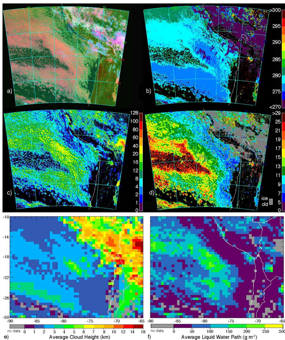
Fig. 10. GOES-10 imagery and retrieved cloud parameters, 15:45 UTC, 27 October 2008: (a) pseudocolor RGB image; (b) cloud effective temperature [K]; (c) cloud optical depth; (d) cloud liquid water droplet effective radius [ \mu\text{m} ]. Regional ( 0.5 \times 0.5^\circ ) average cloud properties, (e) cloud top height, and (f) cloud liquid water path for the same time.
