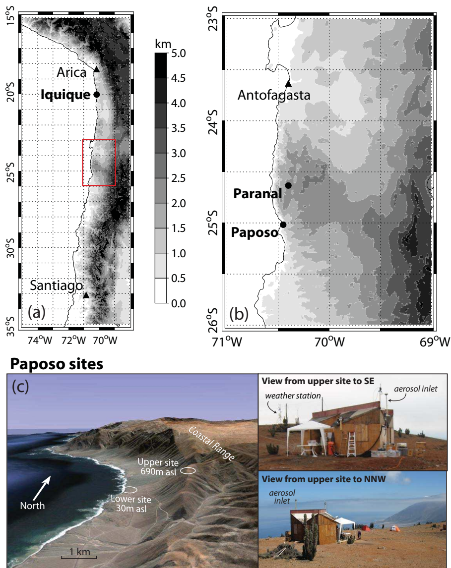
Fig. 4. (a) Map showing location of ground sites used in VOCALS-REx, with (b) a zoomed in map for the red boxed area in (a). Panel (c) shows a Google Earth terrain image showing the Paposos sites looking approximately northward, together with photographs from the upper (elevated) Paposos site.
