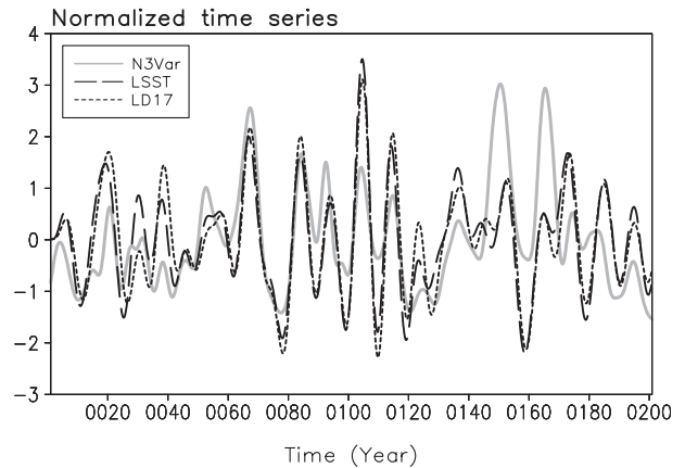
FIG. 3. Gray solid line: time series of the N3Var index. Black short-dashed line: PC time series of first EOF mode for the low-pass-filtered 17°C isotherm depth (see Fig. 2b). Black long-dashed line: PC time series of first EOF mode for the low-pass-filtered SST (see Fig. 2a). Time series has been normalized.
