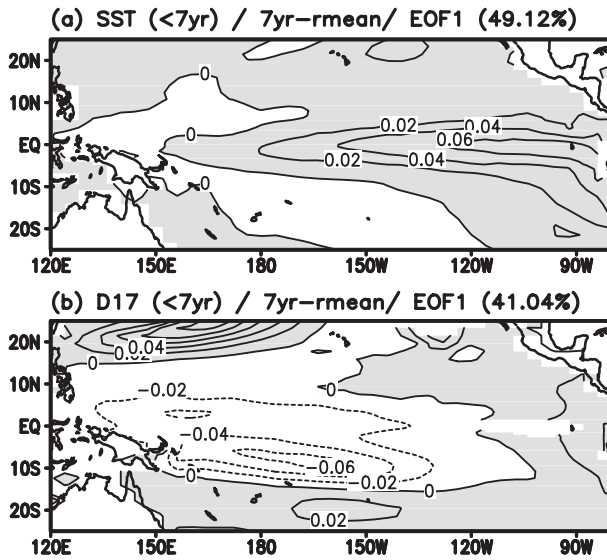
FIG. 8. Spatial pattern of the first EOF mode of (a) the 7-yr running-averaged high-pass-filtered SST and (b) the 7-yr running-averaged high-pass-filtered 17°C isotherm depth anomalies.
