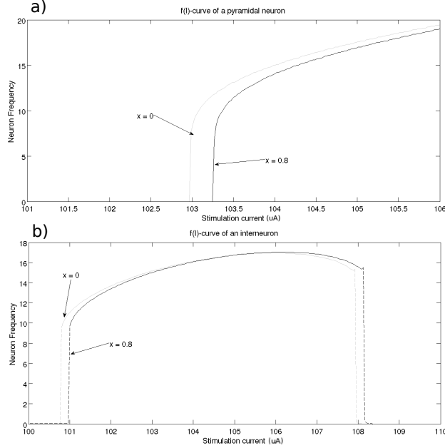
Figure 1: f(I) curves – Effects of tonic inhibition. x represents the amount of tonic inhibition in \mu\text{S} : here g_{ton1} = 20x \mu\text{S} namely 6\mu\text{S} and 16\mu\text{S} , and g_{ton2} = 100x \mu\text{S} namely 30\mu\text{S} and 80\mu\text{S} .
