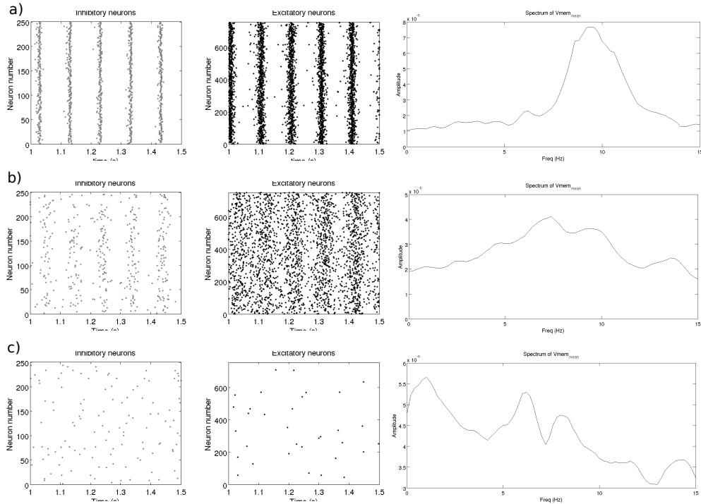
Figure 2: Raster plots of inhibitory and excitatory populations and smoothed power spectrum of the membrane voltage of the excitatory cells: a) without tonic inhibition, b) with tonic inhibition, x = 0.3 , g_{ton1} = 6 \mu\text{S} and g_{ton2} = 30 \mu\text{S} , and c) with x = 0.8 , g_{ton1} = 16 \mu\text{S} and g_{ton2} = 80 \mu\text{S} .
