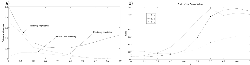
Figure 3: Summary of the effects of tonic inhibition on the synchrony and the subthreshold activity of a cortical neural network. a) Coherence measure of the neuronal population as a function of propofol concentration ( x ). b) Ratio of the power values \delta , \theta and \beta compared to \alpha .
