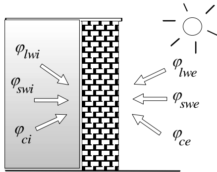
Figure 4 : Boundary conditions
