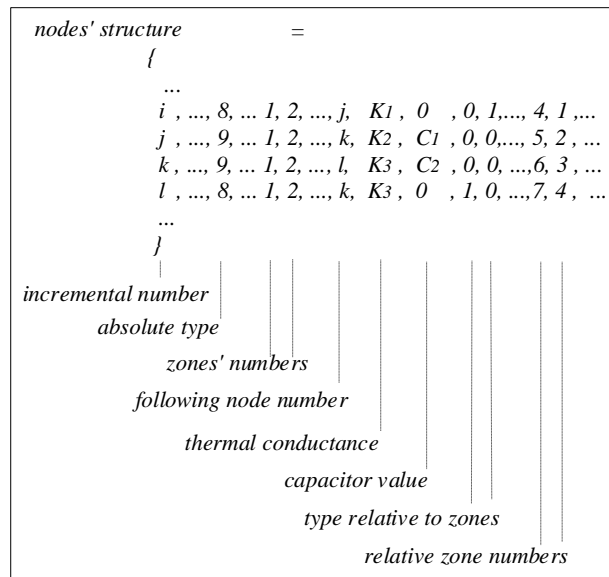
Fig. 13 : Interzone partition and associated data structure
