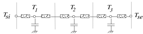
Figure 3 : Associated electrical network
