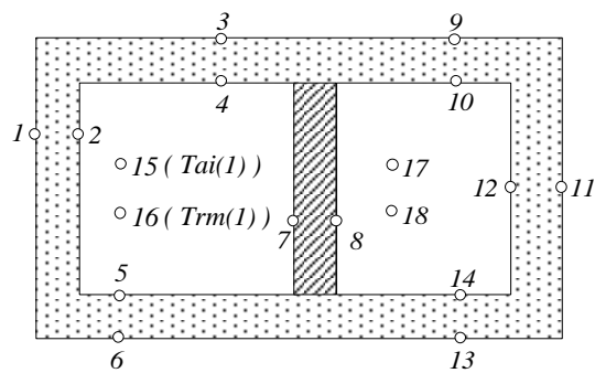
Fig. 9 : Simple two-zone building
