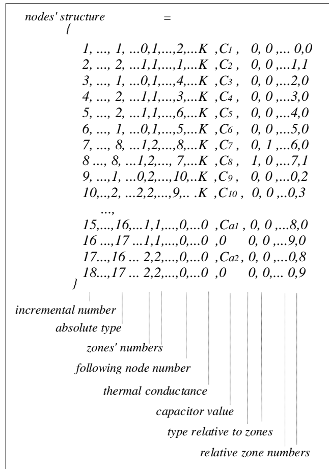
Fig. 14 : Nodes' structure corresponding to fig. 9 building
