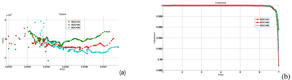
Figure 7. Experimental results with PRBS signal and under several SOCs:- (a) Nyquist plots, (b) coherence plots.
