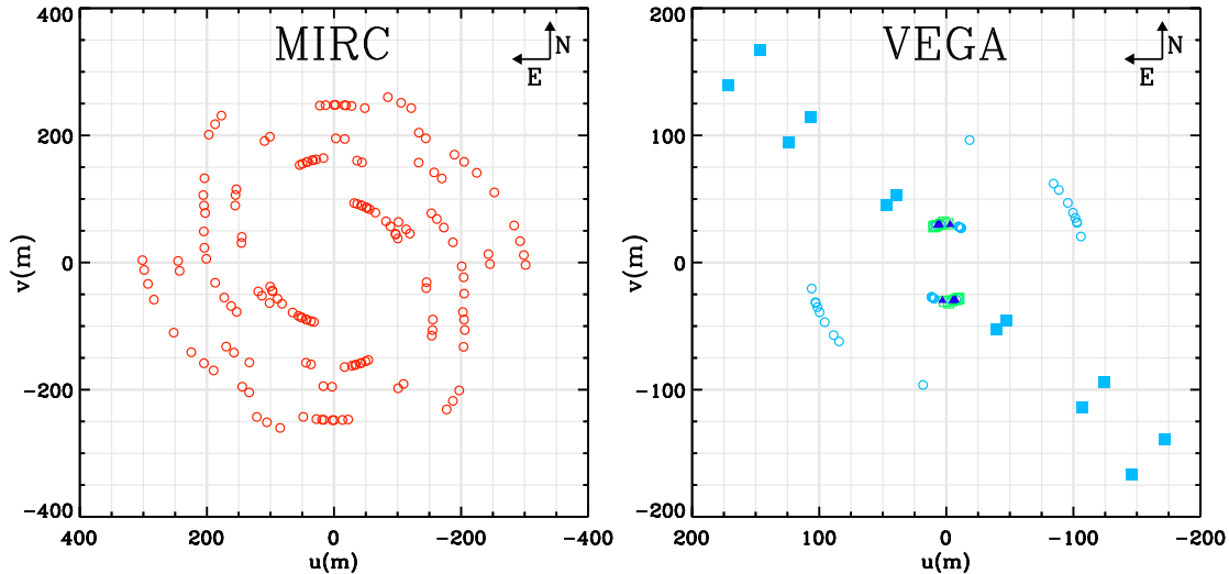
Fig. 1. Left. MIRC/CHARA ( u,v ) plane coverage of \gamma Cas. Right. VEGA/CHARA ( u,v ) plane coverage of \gamma Cas. Blue open circles= 2T MR data, dark blue triangles: 2T HR data, blue square: 3T MR data and green rectangle: 2T polarimetric data
