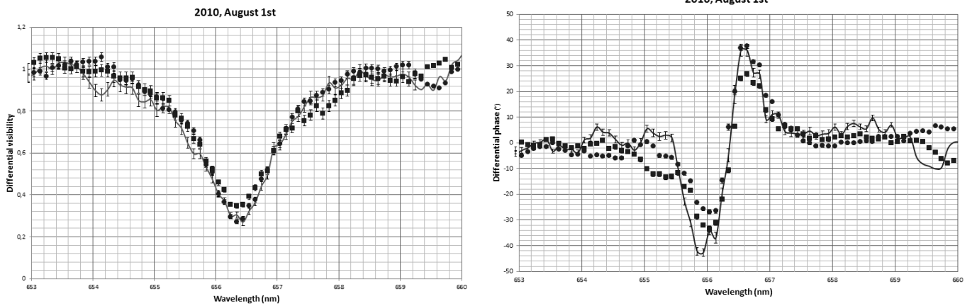
Fig. 7. Differential visibilities (left) and phases (right) obtained on \gamma Cas in natural light (lines), for the linear polarization denoted H (squares) and for the linear perpendicular polarization denoted B (circles) on 2010, August, 1st.
