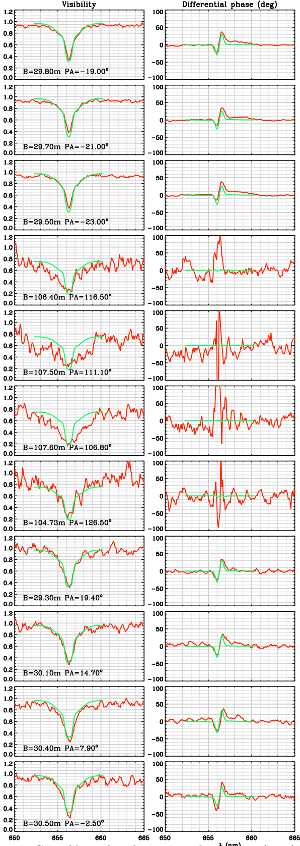
Fig. 5. \gamma Cas calibrated medium spectral resolution (5000) measurements: visibility (left) and differential phase (right) for different baseline length and P.A. indicated on each plot. The visibility and phase from our best-fit model is overplotted in green (plain line).
