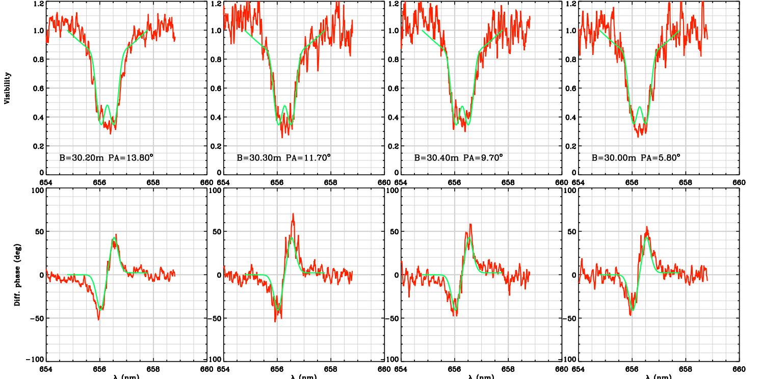
Fig. 8. \gamma Cas calibrated high spectral resolution (30000) measurements: visibility (top) and differential phase (bottom) for different baseline lengths and P.A. indicated on each plot. The visibility and phase from our best-fit model is overplotted in green (plain line).
