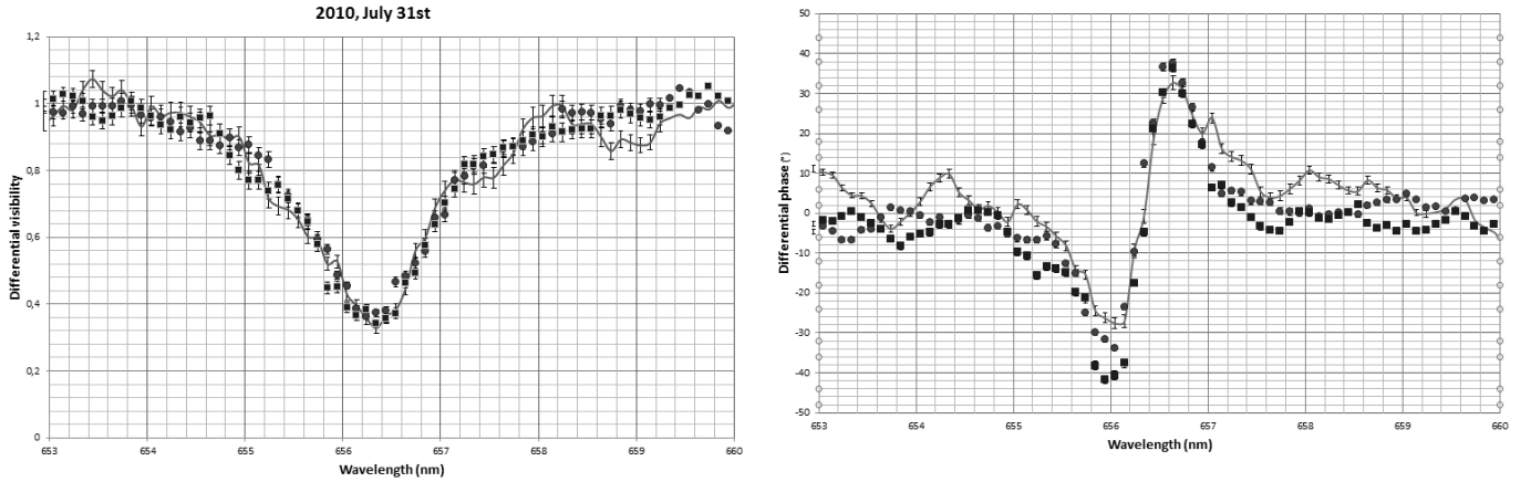
Fig. 6. Differential visibilities (left) and phases (right) obtained on \gamma Cas in natural light (lines), for the linear polarization denoted H (squares) and for the linear perpendicular polarization denoted B (circles) on 2010 July 31.
