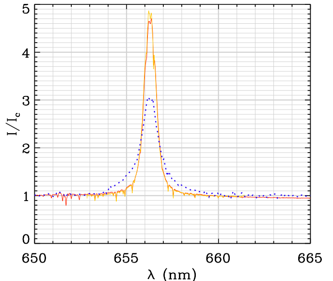
Fig. 2. Medium spectral resolution H\alpha CHARA/VEGA line profiles (blue dotted line) of \gamma Cas, recorded 2008 October 8. Red and yellow solid lines are amateur spectra obtained from the BeSS database, recorded on 2008 September 26 and October, 9.
