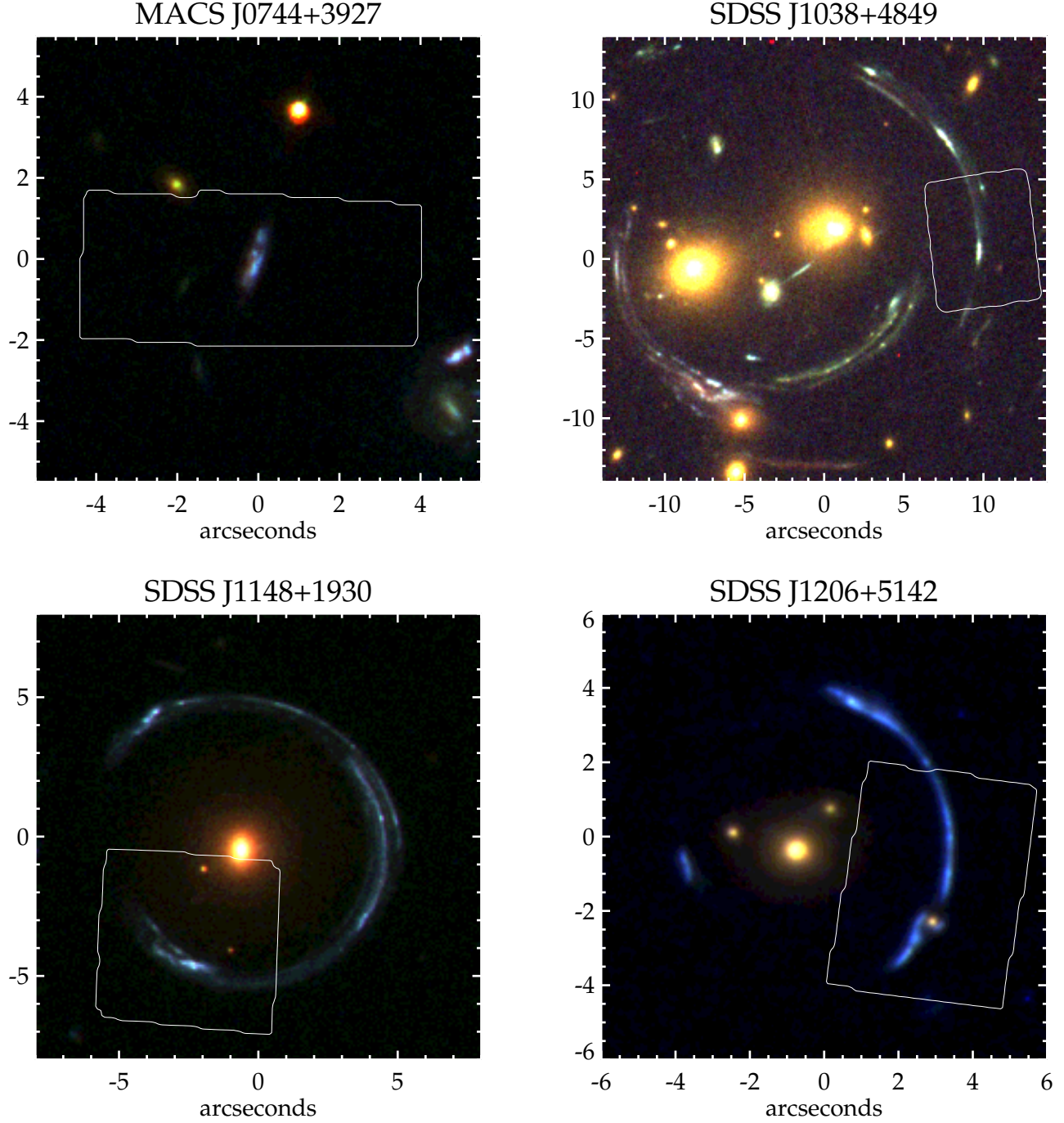
FIG. 1: Color HST images of the sample. The white box in each image shows the OSIRIS field of view used to observe H\alpha and [NII] emission lines. R/G/B channels of each image are respectively ACS F814W/F555W/WFC3 F390W for J0744, WFC2 F814W/F606W/F450W for J1038 and J1206, and WFC3 F814W/F606W/F475W for J1148.
