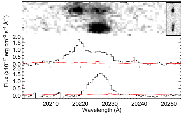
Figure 3. Upper panels: Two-dimensional X-shooter spectrum around the single emission line detected for the M1206 source, and the corresponding region around the source in an HST /ACS/F606W image. The two source IDs 2.1 and 3.1 are separated by 2''.3 and are seen in both panels. Source 2.1 to the North-East in Fig. 1 (upper part in this image) has a compact morphology, and source 3.1 to the South-Western one is more extended. The one-dimensional spectra in the middle and lower panels are extracted for each of the sources and are corrected for telluric absorption lines.
