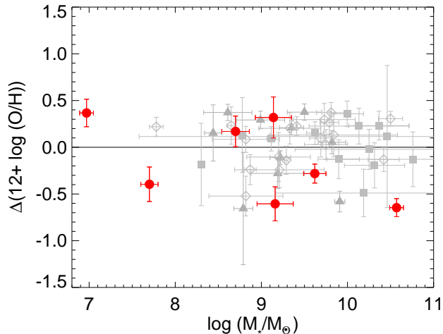
Figure 9. Offset in measured abundance compared to the new calibration of the fundamental relation given by Eq. (1). The symbols present the same data as in Fig. 8. From the entire sample of lensed galaxies combined with low redshift GRB hosts, we measure a standard deviation of \sigma = 0.3 dex.
