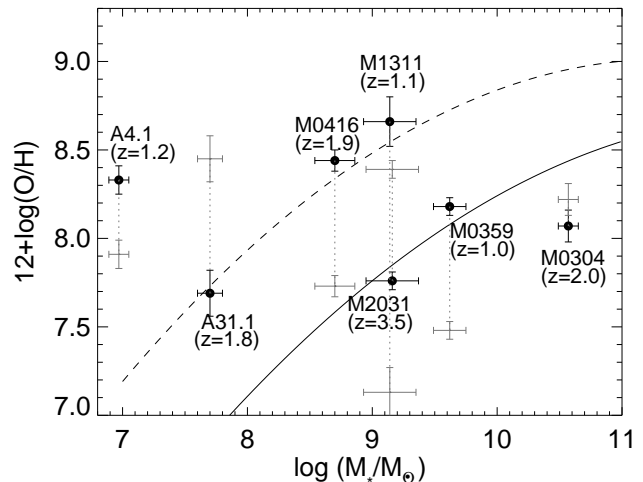
Figure 7. Oxygen abundances of the lensed galaxies as a function of the stellar masses, corrected for lens magnifications. The black circles show the oxygen abundances from the preferred branch of the R_{23} relation including the direct measurements for A31.1, M0304 and M2031, while the grey error-bars show the location of the galaxies if the alternate branch of the R_{23} relation is adopted for all galaxies. The mass-metallicity relation for Lyman break galaxies at z = 3 - 4 is shown by the solid line (Maiolino et al. 2008; Mannucci et al. 2009), and galaxies at z = 0.7 by the dashed line (Savaglio et al. 2005).
