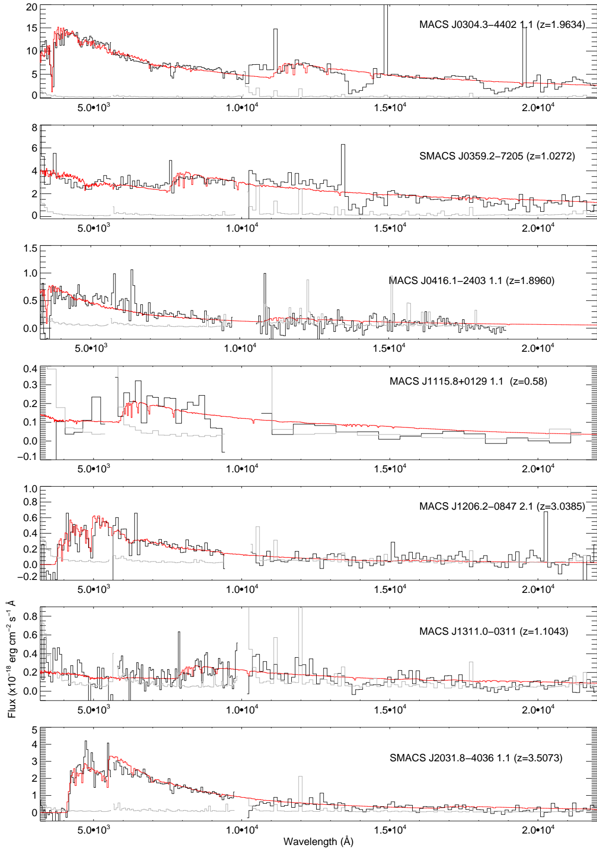
Figure 2. Binned source spectra with the best fit spectral templates overlotted by the red lines (Sect. 4.1). The grey lines are the error spectra. Regions with very noisy data are omitted, both in the fitting and in the display. In particular, wavelengths at 1\mu\text{m} between the VIS and the near-IR arm are dominated by uncertainties in the flux calibration. See the electronic issue of the paper for a colour version of this figure.
