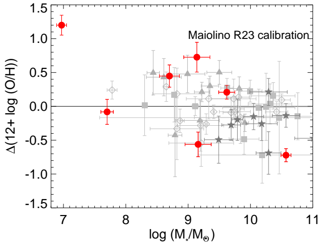
Figure 8. Offsets of the derived oxygen abundance compared to the predicted one from the fundamental relation in Mannucci et al. (2011). The red circles show the location of the preferred R_{23} branch with the calibration in Maiolino et al. (2008), and using the direct measurements for A31.1, M0304 and M2031 in Christensen et al. (2012). A location above zero implies that the measured metallicity is higher than expected from the relation. The grey squares show the offsets of 13 lensed galaxies at z = 2 - 3 for which either the R_{23} or the N2 calibration from Maiolino et al. (2008) were used (Richard et al. 2011a). The grey triangles show offsets of 10 lensed galaxies at z = 1 - 2 in Wuyts et al. (2012b) for which the oxygen abundance was derived from the N2 calibration in Maiolino et al. (2008). The outlined diamonds represent 18 GRB hosts at z < 1 (Mannucci et al. 2011), and the star symbols represent unlensed and more massive z \sim 3.5 galaxies (Maiolino et al. 2008).
