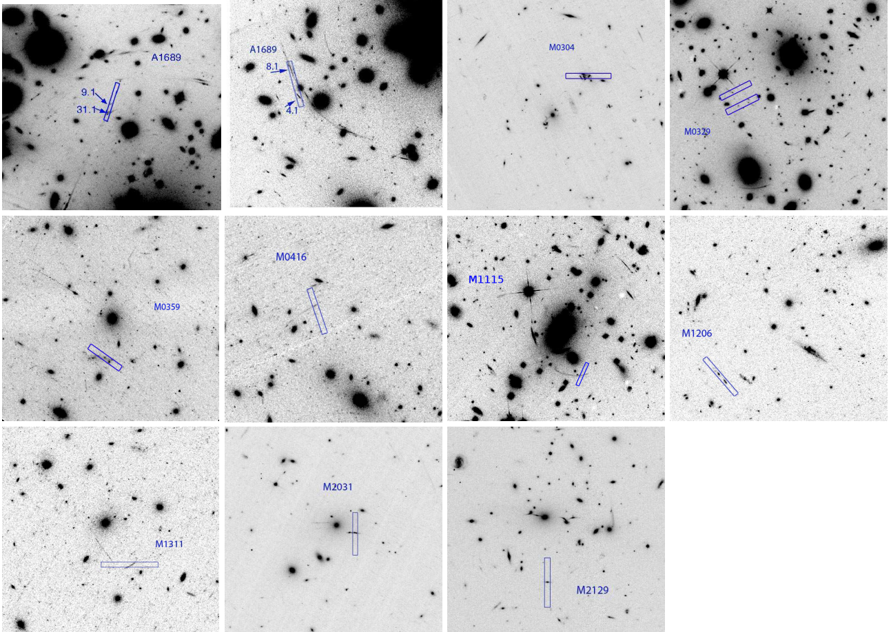
Figure 1. Thumbnail HST images of the clusters around the targeted sources. The images were taken with ACS, WFCP2 or WFC3 with either the F606W, F814W or F110W filters, and obtained through the MAST or HLA data archive ( http://hla.stsci.edu/ ). The images have varying sizes between 40 and 90 arcsec on a side with the orientation North up and East left, and with the X-shooter 11'' slit position indicated.
