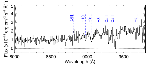
Figure 5. Section of the VIS and near-IR spectra of the M2129 arc ID 1.5 binned to a dispersion of 5.2 and 12 Å pixel -1 , respectively. Detections of Ca II 3934,3969 lines and absorption lines from the Balmer series of hydrogen at z = 1.3617 are indicated. Also a faint emission line from the [O II] \lambda 3727 doublet is visible in this binned version.
