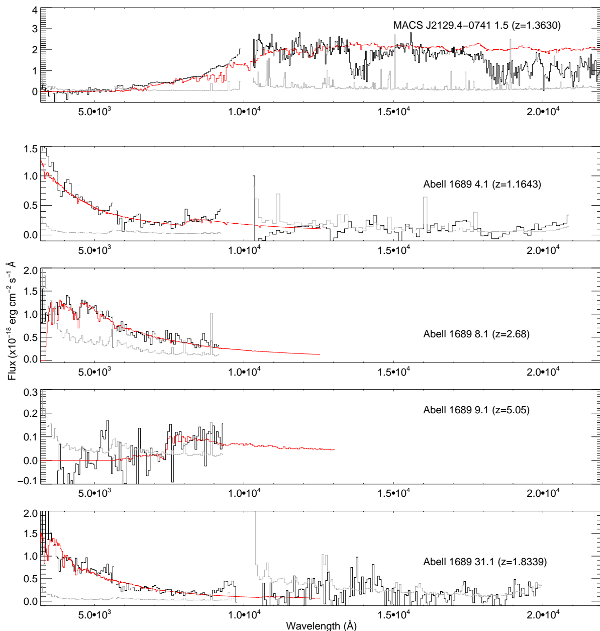
Figure 2. – continued. The continuum emission in the near-IR for the Abell 1689 arcs, is considerably more noisy compared to the other spectra due to increased sky subtraction errors.
