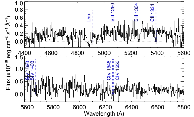
Figure 4. Section of the UVB and VIS spectra of the M1206 source ID 2.1 binned by 10 and 20, respectively, to a dispersion of 2.5 \text{ \AA pixel}^{-1} . Typical strong UV absorption lines seen in high redshift galaxies are marked at the redshift z = 3.0385 .
