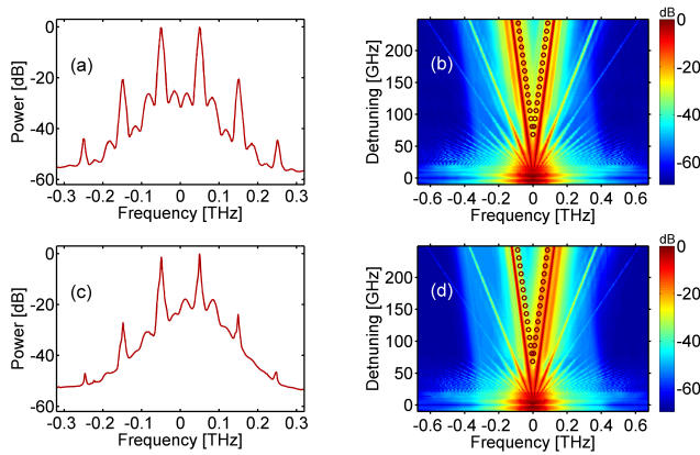
Fig. 2. (a-c) Experimental output spectra showing MI developing over mFWM for balanced (a) and imbalanced (c) pumps at \Delta f_p = 100 GHz and P = 800 mW. (b-d) color maps of output spectrum as a function of detuning \Delta f_p ranging from -10 to 250 GHz, measured in the balanced (b) and imbalanced (d) case. Open dots correspond to the most unstable frequency f_{MI} from theory.
