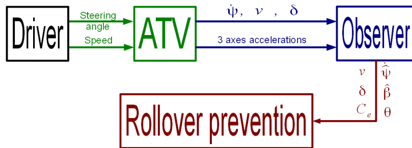
Figure 2: Algorithm overview.
