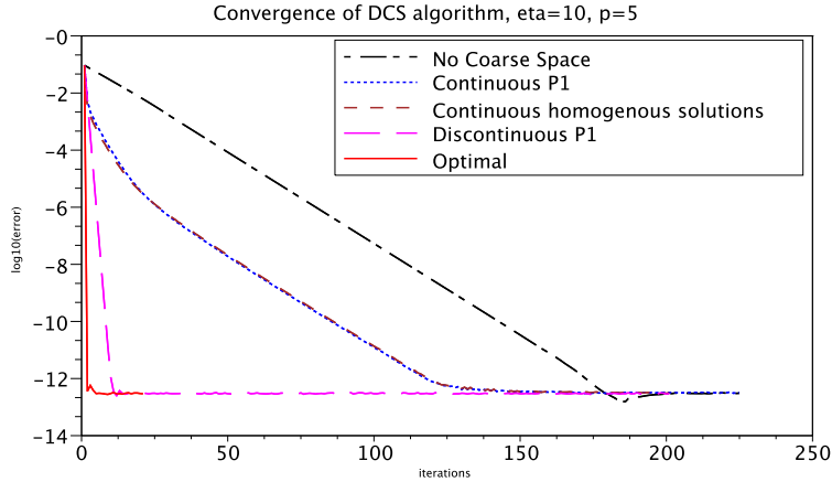
Fig. 1 Convergence curves of the DCS-DMNV algorithm in 1D
