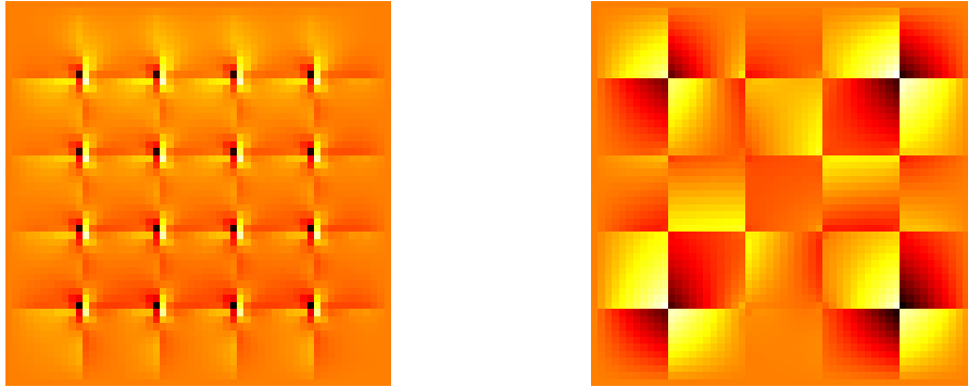
Fig. 3 Error of the algorithm with continuous coarse grid correction at iterations 5 and 20
