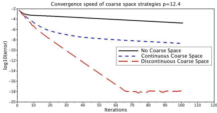
Fig. 2 Convergence curves of the DCS-DMNV algorithm in 2D
