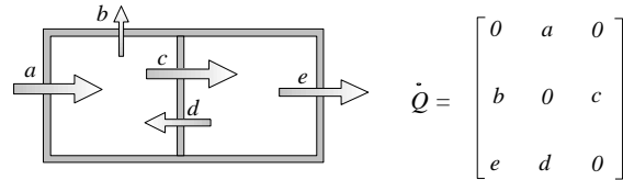
Fig. 4 : Interzonal airflow rates matrix
