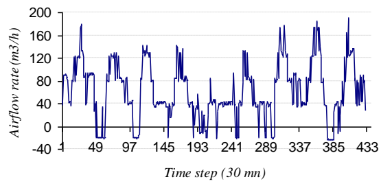
Fig. 12 : Incoming air flow in the living room
