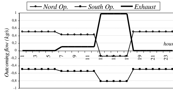
Fig. 9 : Evolution of outcoming airflows
