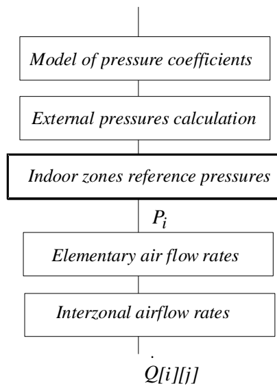
Fig. 6 : Flow chart for airflow rates calculation
