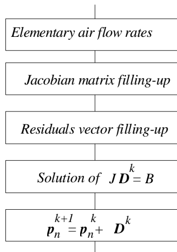
Fig. 8 : Pressure calculation flow chart
