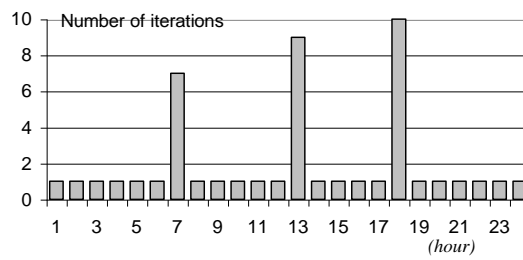
Fig. 10 : Required iterations
