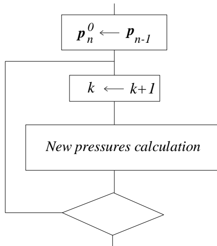
Fig. 7 : Non linear pressure system solution
