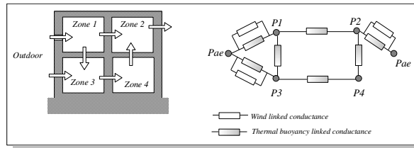
Fig 2 :Airflow network
