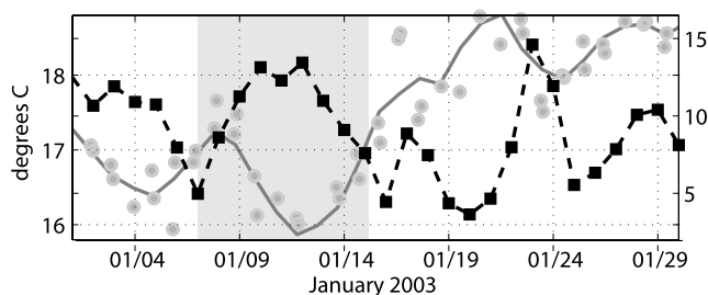
Figure 12. A detailed view of the temporal variation of ocean temperature and surface wind during the January 2003 CJ event. Gray dots show the sea surface temperature estimated by TMI at ( 73.2^{\circ}\text{W} , 30.1^{\circ}\text{S} ). Solid lines show the SST variation (a low-pass filter ( f_c = 3\text{ d}^{-1} ) was applied). The daily mean QuikSCAT wind speed estimates at the same location as the TMI data are also shown (dark squares connected by dashed line).
