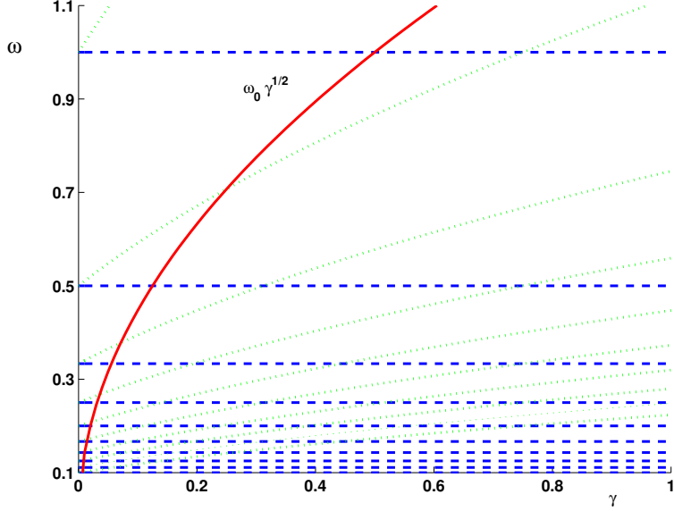
FIGURE 3. Resonance tongues on the plane (\gamma, \omega) (delimited by dotted and dashed lines), and breather frequency curve \omega = \sqrt{\gamma}\omega_0 (solid line) for \kappa = 1 . No resonances occur for \gamma \in \cup_{m \geq m_0} (\Gamma_m, \gamma_m) , where \Gamma_m and \gamma_m correspond to the intersections of \omega = \sqrt{\gamma}\omega_0 with \omega = \frac{\sqrt{\kappa^2 + 4\gamma}}{m} (dotted lines) and \omega = \frac{\kappa}{m} (dashed lines) respectively.
