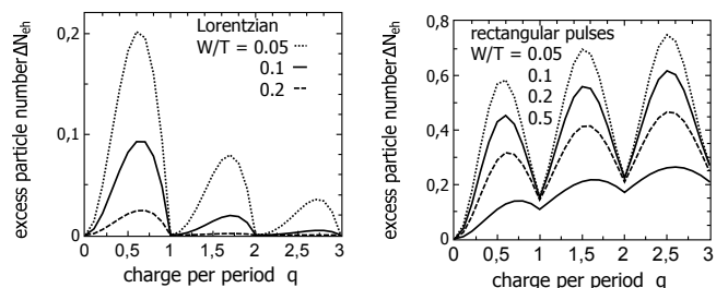
FIG. 7: Excess electron and hole particle number for Lorentzian (left) and rectangular (right) pulses carrying q charges per period and for different width to period ratio W/T
