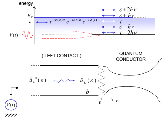
FIG. 1: Under the effect of a ac voltage, electrons emitted far inside the contact acquire a time dependent phase on their way to the scattering region (the quantum conductor). For periodic voltage, frequency \nu , the incoming electrons can be described by a quantum superposition of states at different energies \epsilon + lh\nu .
