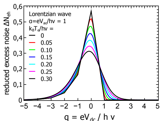
FIG. 13: Finite temperature excess electron and hole particle noise versus dc voltage in reduced units for Lorentzian waves of amplitude \alpha = 1 .
