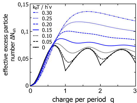
FIG. 8: Effective excess electron and hole particle for sine pulses carrying q charges per period and for different electron temperature T_e
