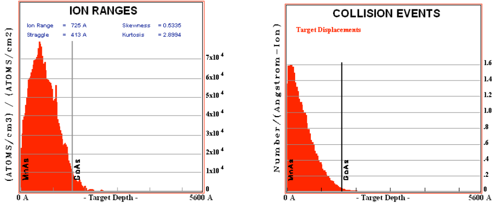
Figure 3: SRIM predictions [12] on the ion penetration and collision events with the present experimental conditions: \text{Ne}^{9+} at 90 keV on MnAs/GaAs (150 nm) with an incidence angle of 60^\circ . Left: distribution of the ion penetration. Right: distribution of atom displacement in the sample. As we can observe, only a very small fraction of ions is deposited in the GaAs substrate.
