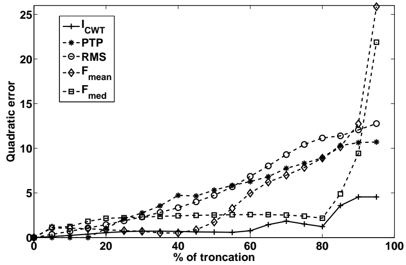
FIGURE 8 – Error of fatigue algorithms results ( I_{CWT} , PTP, RMS, F_{mean} and F_{med} ) for different level of truncation
