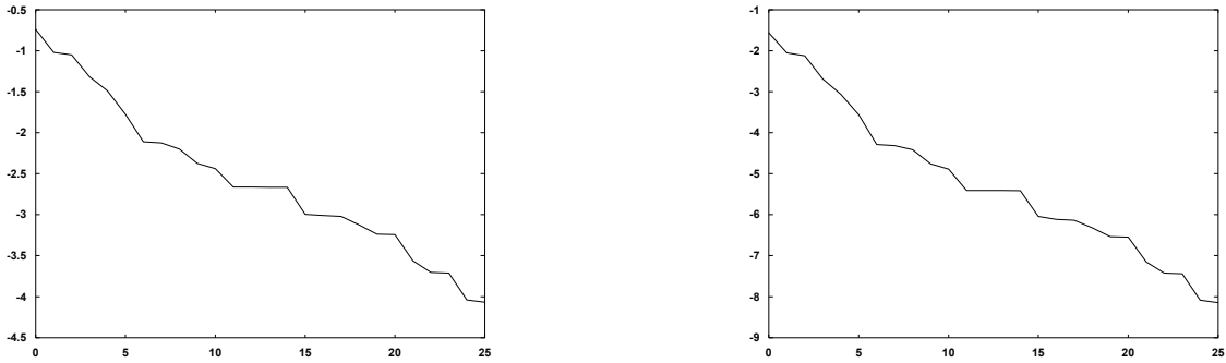
FIG. 3.2. \mathcal{B}_n and \mathcal{C}_N in logarithmic scale with respect of N
