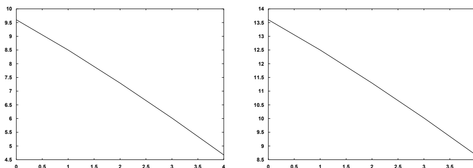
FIG. 5.11. \mathcal{A}_N with respect of N , with \zeta = 1e - 10 (left) and \zeta = 1e - 14 (right)
