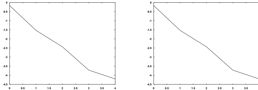
FIG. 5.3. \mathcal{A}_N with respect of N , with \zeta = 1e - 10 (left) and \zeta = 1e - 14 (right)
