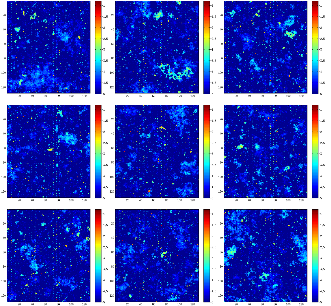
FIGURE 12. Simulations of \mu_N^{f_3} on grids E_N , with N = 20000, \dots, 20008 (from left to right and top to bottom)
