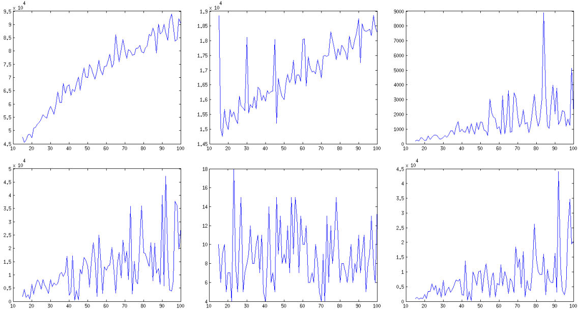
FIGURE 6. Size of the maximal invariant set \Omega((f_i)_N) (left), number of periodic orbits of (f_i)_N (middle) and length of the largest periodic orbit of (f_i)_N (right) depending on N , for f_1 (top) and f_2 (bottom), on the grids E_N with N = 128k , k = 15, \dots, 100
