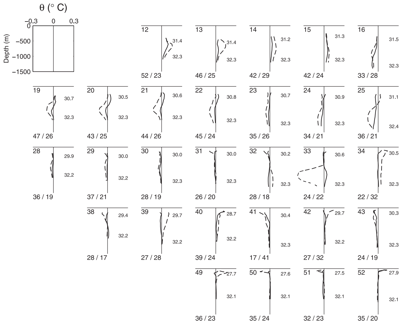
Figure 3. The first two bivariate isopycnal EOFs defined as departures from RLMB climatology: potential temperature ( ^{\circ}\text{C} ) and isopycnal displacement (in meters) as a function of depth (in meters). The percentage of variance explained (PVE) estimates (lower left) given by \text{PVE}(\lambda) = 100 \times \lambda / \sum_{m=1}^{2K} \lambda_m and the first (upper right) and last (lower right) \sigma levels ( \text{kg}/\text{m}^3 ) of the isopycnal grid are indicated for each bin. The first mode is shown as a solid line, and the second one is dashed. In bins 34, 39, 41, and 42 we have intentionally reversed modes 1 and 2.
