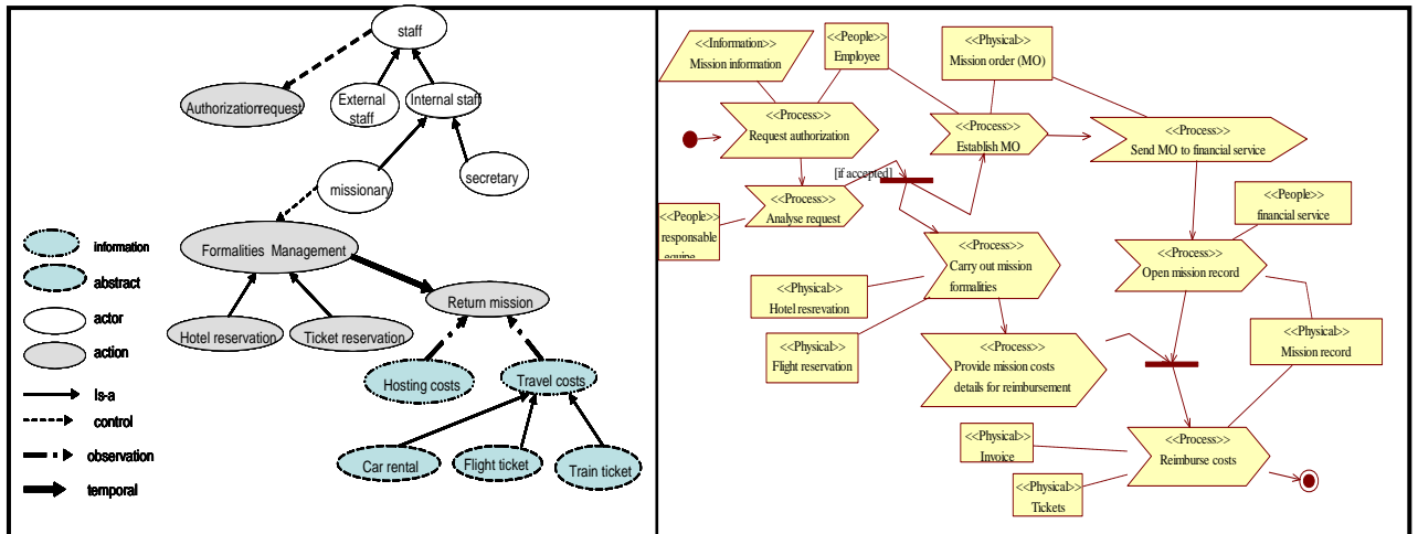
Fig. 1 Instantiation of the BPM meta model and of the Ontology meta-model
