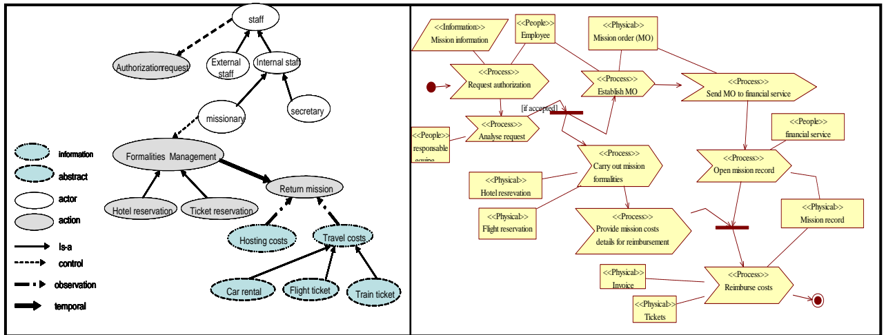
Fig. 1 Instantiation of the BPM meta model and of the Ontology meta-model
