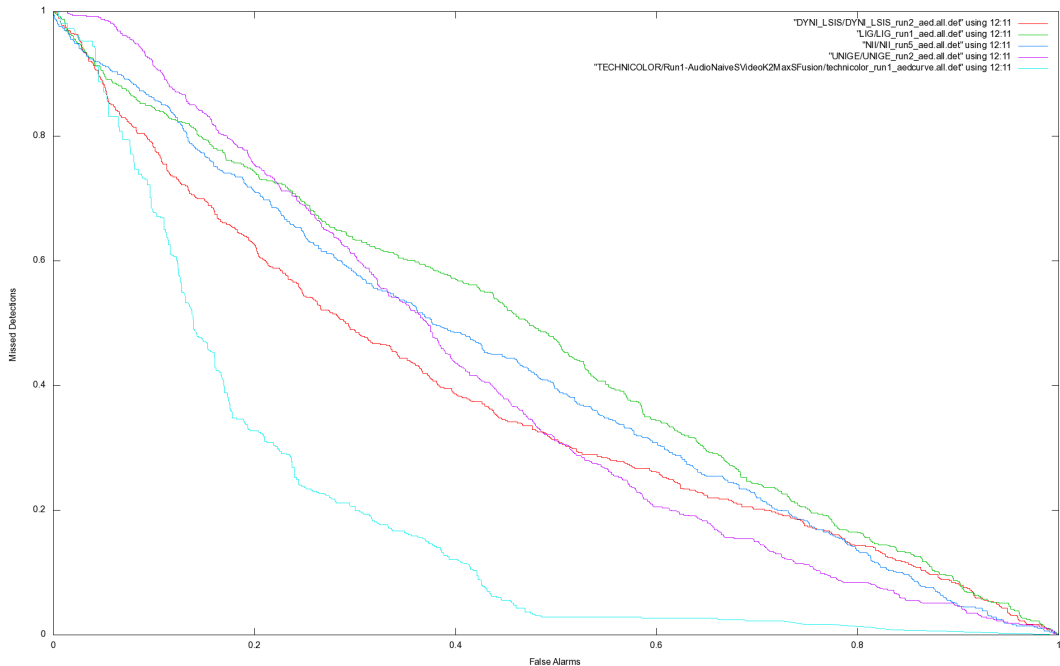
Figure 1: False alarms' rate versus miss rates for participants' best runs
