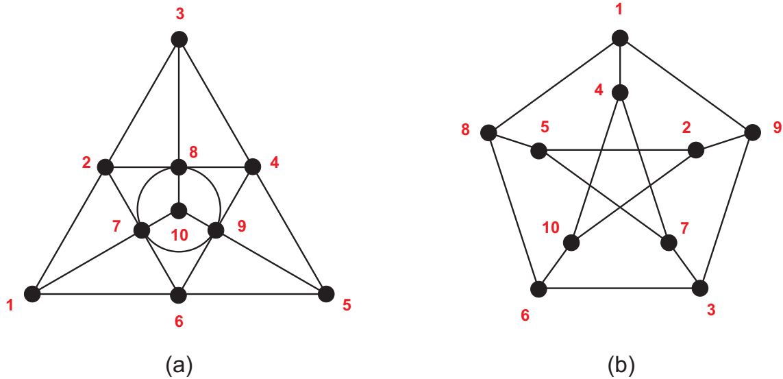
Figure 2. (a) The non-realizable 10_3 -configuration and (b) the complement of its collinearity graph, the Petersen graph.
