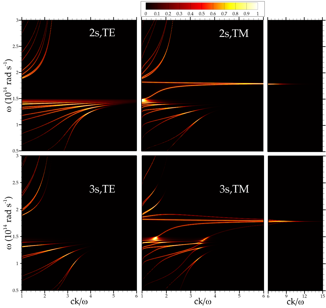
FIG. 1: Two- (upper side) and three-body (lower side) transmission probabilities for both polarizations as a function of \omega and k at separation distance d = 700 nm and \delta = 870 nm.
