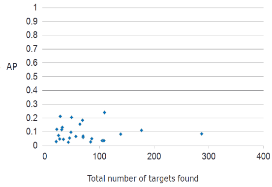
Figure 31: AP vs. number found (automatic)
