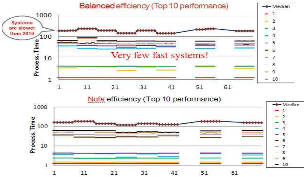
Figure 42: Top 10 runs efficiency in both profiles
