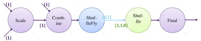
Fig. 6: A model of idct with the ratios of tokens productions and consumption.
