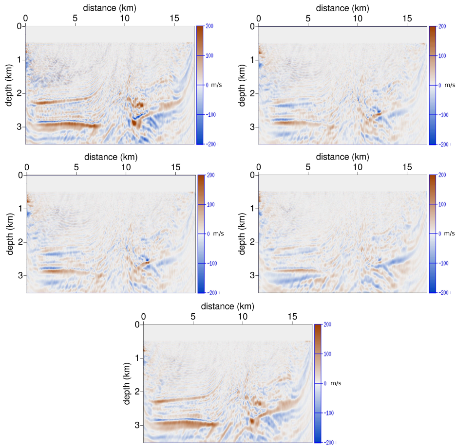
FIG. 4.7. Difference between the l-BFGS estimated model and the other estimated models. Newton (top left), Gauss-Newton (top right), outer preconditioned Newton (middle left), outer preconditioned Gauss-Newton (middle right), steepest-descent (bottom)
