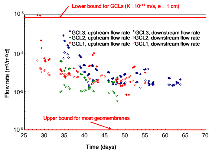
Figure 9. Synthesis of flow rates obtained for multicomponent GCLs
