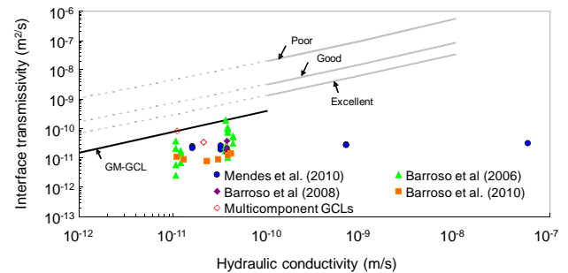
Figure 12. Synthesis of transmissivity data obtained in the literature for GCLs in contact with geomembranes and for multicomponent GCLs.
