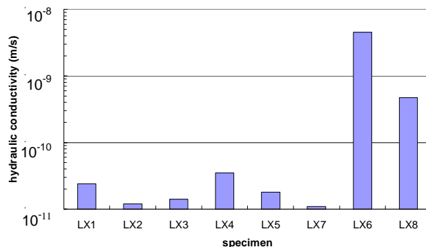
Figure 4. Hydraulic conductivity to NaCl 10^{-3} M of GCLs LX1 to LX8 from Guyonnet et al. (2009)
