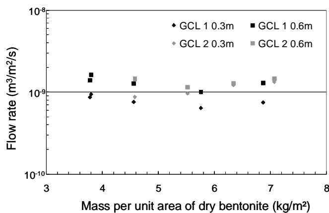
Figure 5. Evolution of the flow rate in two GCLs as a function of the dry mass per unit area of bentonite
