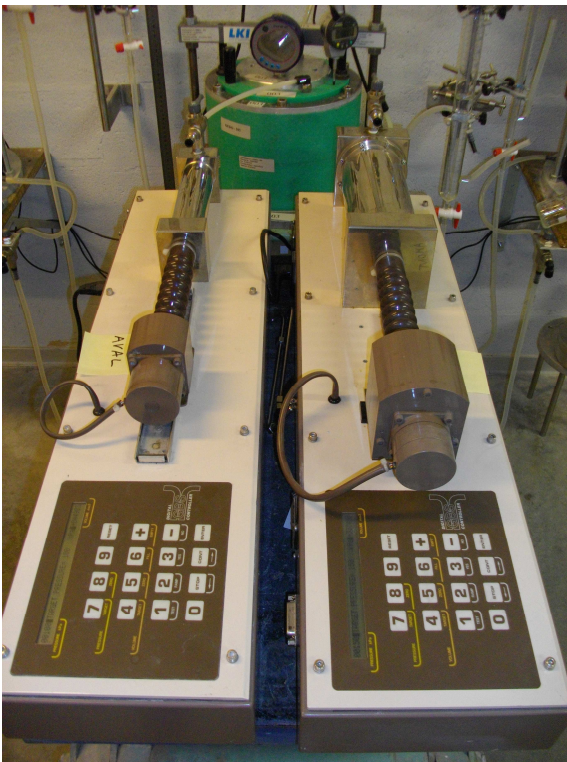
Figure 8. Experimental device for measurement of flow rates through multicomponent GCLs
