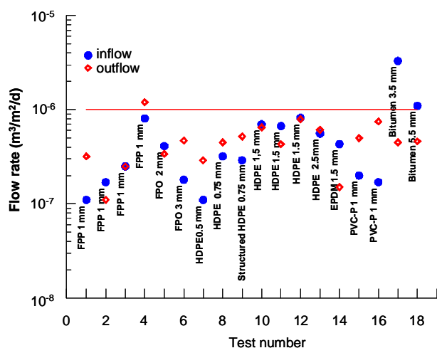
Figure 2. Synthesis of flow rate measurements through geomembranes according to EN 14150 with Type B device (from Touze-Foltz & Zanzinger 2009) (FPP: flexible polypropylene, EPDM: ethylene propylene diene monomer, HDPE: high density polyethylene, PVC-P: plasticized polyvinyl chloride, FPO: flexible polyolefine)
