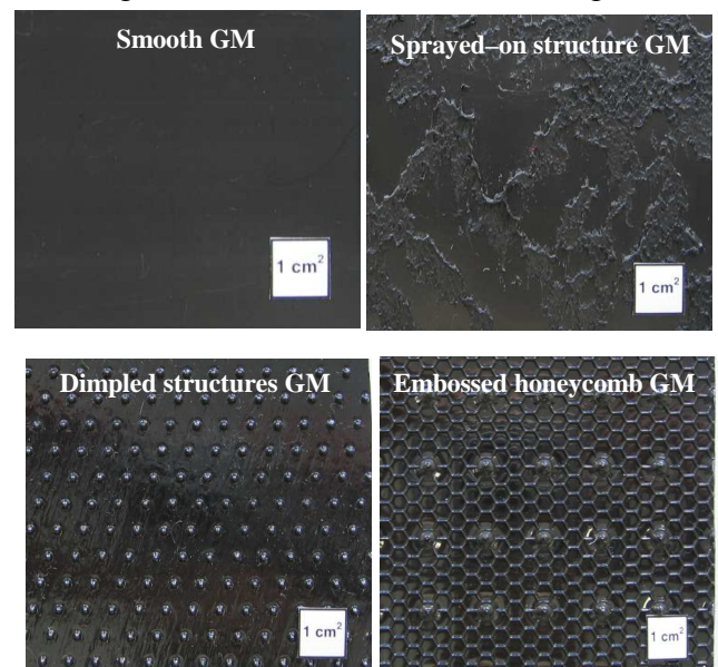
Figure 10. Types of textured geomembranes used in the study by Barroso et al. (2008)
