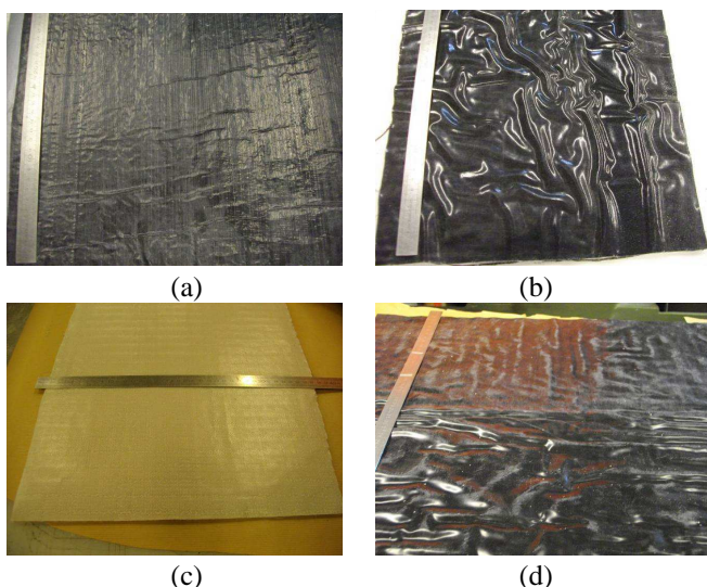
Figure 11. View of the surface of the various coated GCLs studied: (a) GCL1, (b) GCL2, (c) GCL3, and (d) GCL4.
