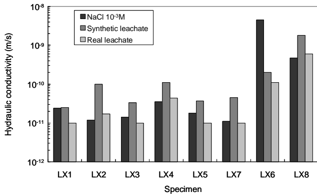
Figure 14. Values of hydraulic conductivity measured by Guyonnet et al. (2009) on 8 different GCLs under a 100 kPa load with various fluids
