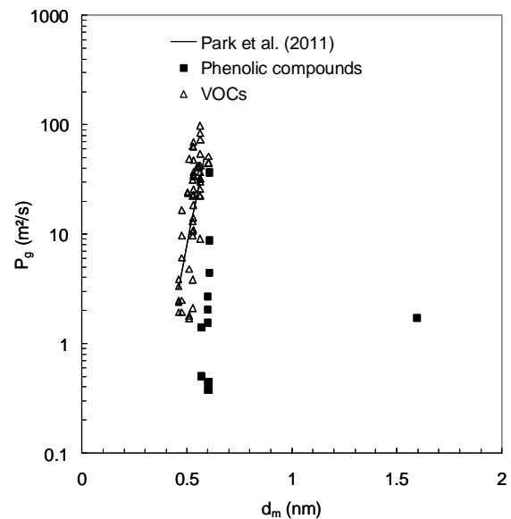
Figure 17. Relationship between permeation coefficient, P_g , and: (a) aqueous solubility, (b) octanol-water partition coefficient, K_{ow} , and (c) molecular diameter, d_m for phenolic compounds and VOCs (adapted from Touze-Foltz et al. 2012).
