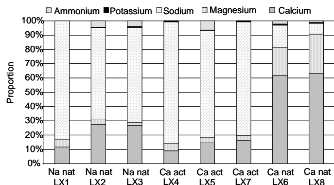
Figure 3. Main cation proportion in the various GCLs LX1 to LX8 tested by Guyonnet et al. (2009)
