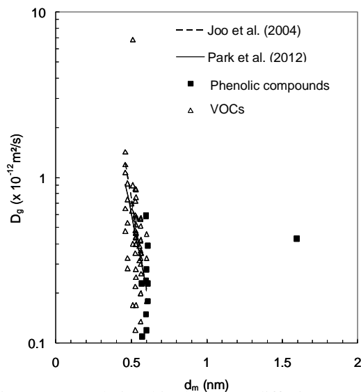
Figure 16. Relationship between diffusion coefficient, D_g , and: (a) aqueous solubility, (b) octanol-water partition coefficient, K_{ow} , and (c) molecular diameter, d_m for phenolic compounds and VOCs (adapted from Touze-Foltz et al. 2012).
