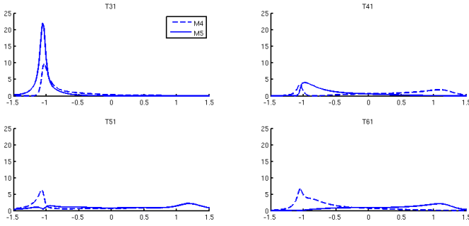
Fig. 9. Stored energies for second to forth resonator and for both solution M^4 and M^5
