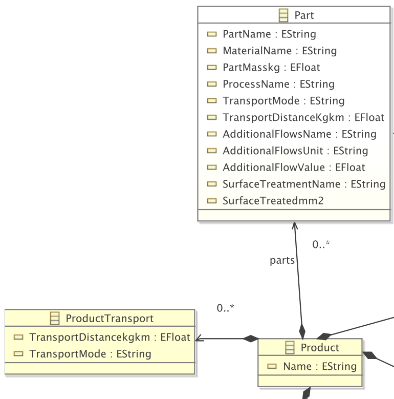
Figure 2: Extract of the UML model to describe the environmental analysis inputs needed to perform an LCA
