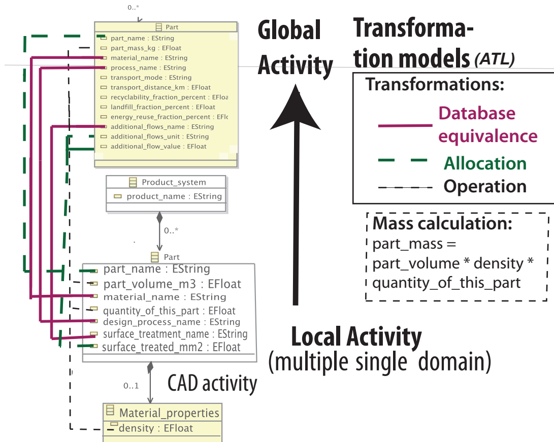
Figure 6: Example of knowledge transformation models between (1) structural designer activity outputs (2) logistic activity outputs and (3) environmental engineer activity inputs
