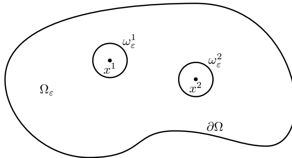
Figure 1: The perturbed domain when N = 2 .
