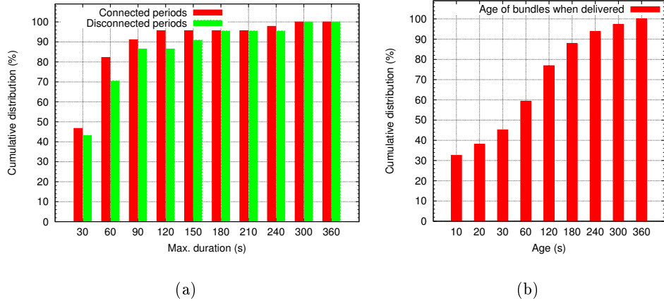
Fig. 4. Cumulative distribution (a) of hotspot connectivity periods, and (b) of the age of bundles at delivery time
