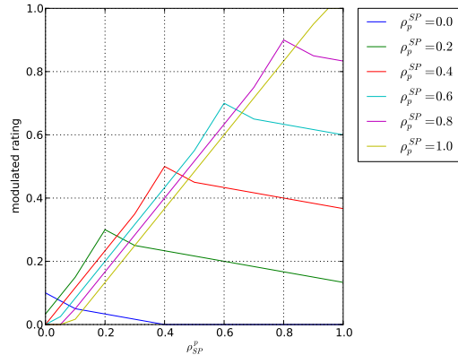
Figure 5: Correlation function
