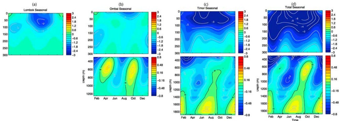
Figure 5. Seasonal cycle of transport per unit depth ( 10^{-2} \text{ Sv m}^{-1} ) for (a) Lombok Strait, (b) Ombai Strait, (c) Timor Passage, and (d) the total transport to the respective sill depths. Note change of vertical and transport scale for depths of >300 \text{ m} .
