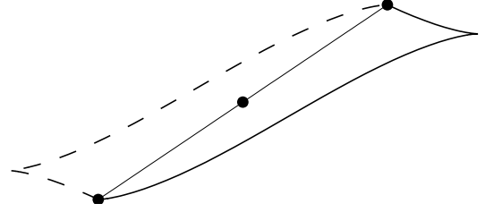
Figure 10: Action of \mathbb{T} on t \mapsto (x(t), y(t)) .
