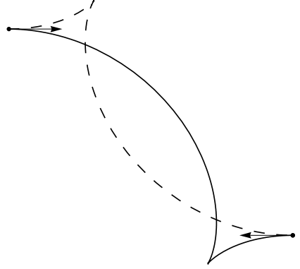
Figure 12: Maxwell point for reflection \mathbb{T} .
