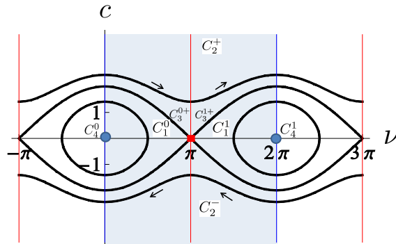
Figure 5: Phase portraits of the pendulum equation, with the 5 types of trajectories.
