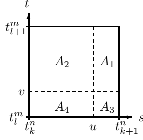
Figure 1. Decomposition of rectangle J_{k,l}^{n,m} for a fixed (u, v) \in J_{k,l}^{n,m} used in the integration (**).
