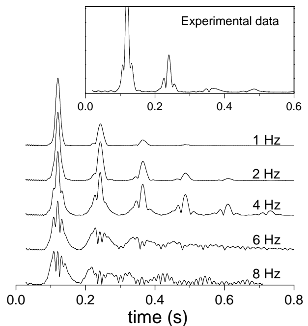
Figure 6: Main plot: numerical 3D lattice simulations of the variation of the echo pattern as a function of f_{dip} for \tau = 120 ms (with slice-selection and taking into account xenon diffusion). Inset: experimental result with a dissolved laser-polarized xenon sample ( f_{dip} = 9 Hz). The vertical scale is chosen so as to better visualize the altered echo shapes.
