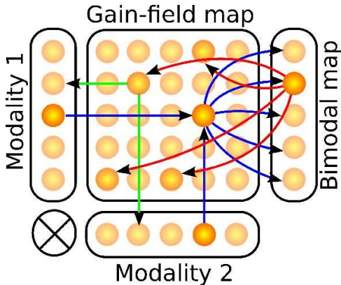
Fig. 2. Reentrant mechanism. The unimodal neurons fed univocal sensory signals to the gain-field neurons and to the downward neurons, and receive back the multimodal response; adapted from [22], [13] and [23].
