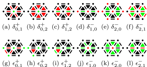
Figure 5: Dimensional operators.
