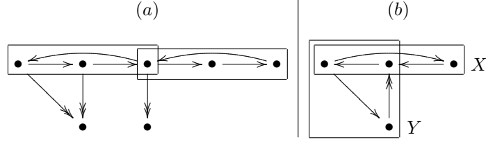
Figure 1: Examples of sources of conflict. Single arrow arcs depict the \nearrow relation and double arrow arcs depict the immediate successors of relation < .
