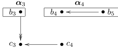
Figure 3: Illustrating the future of W_U = \{a_2, a_4\} in AES from Figure 2. The branching cells \alpha_3 and \alpha_4 are depicted by frames.
