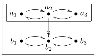
Figure 5: An AES with two non empty CC-prefixes which are framed. The configuration \{a_1, a_3, b_1\} is a CC-configuration.
