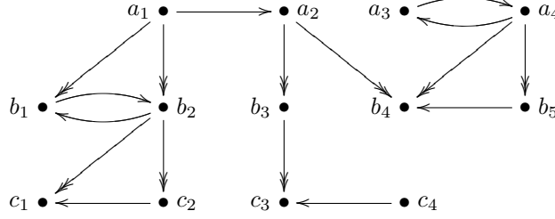
Figure 2: An example of AES.
