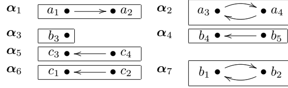
Figure 4: All non empty branching cells of the AES depicted in Figure 2.
