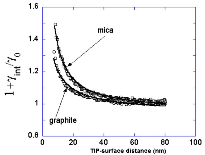
FIG. 2. (Color online) The damping coefficient extracted from the amplitude data. The solid lines are fits to the data using the expression given in the text.
