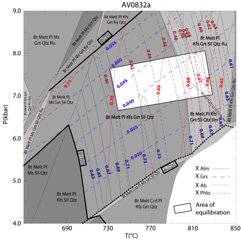
Fig. 10. P-T pseudosections of garnet-bearing migmatite AV-08-32a in the NCKFMASHT system. Isoleths of almandine ( X_{Alm} ), grossular ( X_{Grs} ), phlogopite ( X_{Phlo} ) and albite ( X_{Ab} ) are plotted in the field of the observed peak P-T mineralogical assemblage; the white box represent the P-T conditions of garnet, biotite and plagioclase equilibration; i.e., when measured composition matches the theoretical composition constructed by isopleths. Bulk compositions used for each pseudosection are reported in Table 7. Same shading as Fig. 8.
