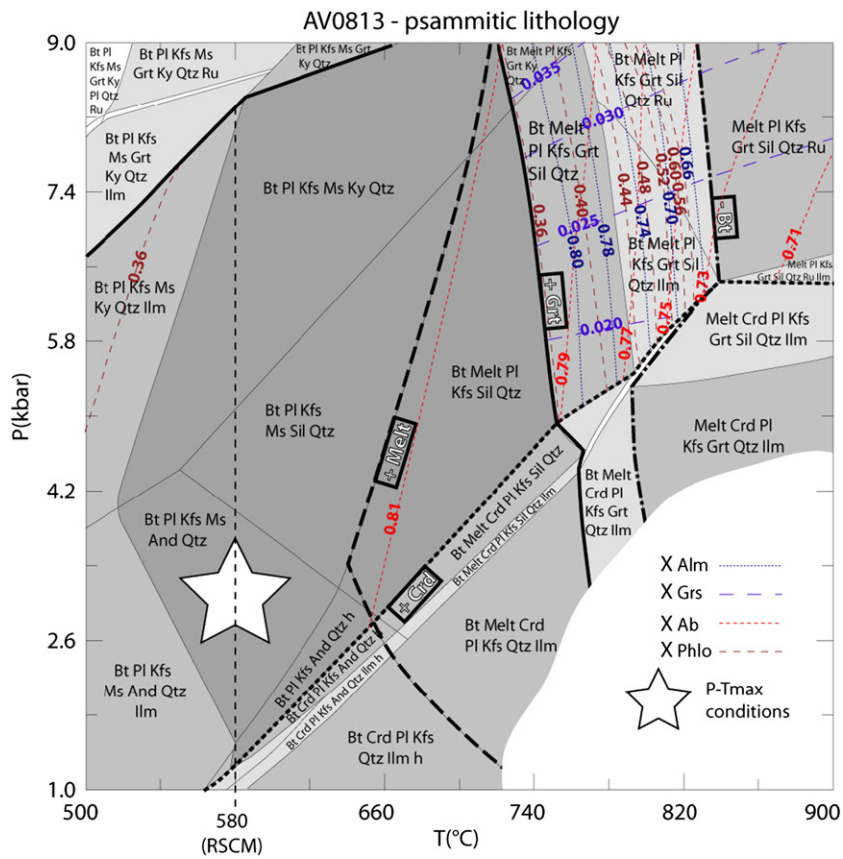
Fig. 1. P - T pseudosection of AV-08-13 metapsammite sample in the NCKFMASHT system. The white star corresponds to P - T_{max} metamorphic conditions underwent by the sample. These conditions have been estimated using the observed paragenesis and RSCM thermometry. Estimated conditions are supported by the compositions of biotite and plagioclase. The heavy black arrow represents the suggested P - T path before P - T_{max} conditions based on aluminosilicate sequence of Fig. 5a & b. Bulk compositions used for each pseudosection are reported in Table 5. No shading = field divariant, then light to dark shading = increasing the variance (trivariant, quadrivariant, etc.).
