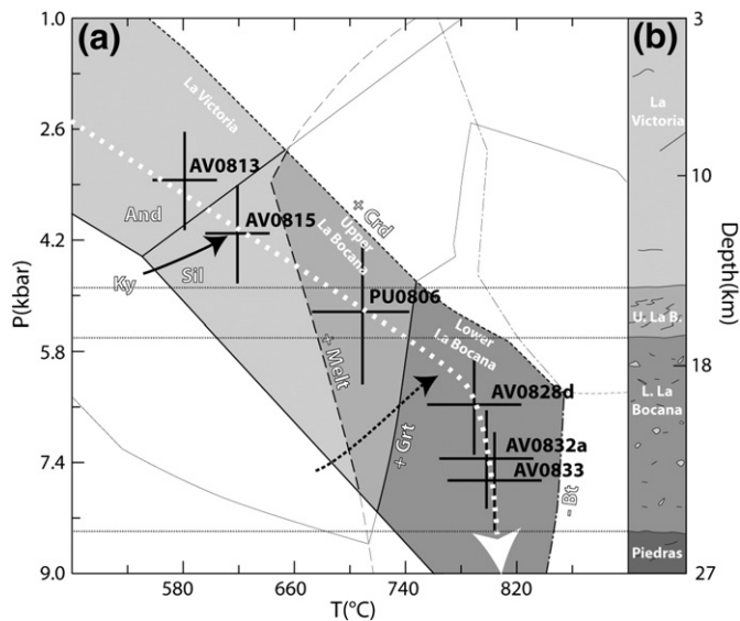
Fig. 12. P-T diagram for El Oro metamorphic complex. (a) reported peak P-T max conditions of studied samples in the simplified pseudosection of AV-08-15 sample (Fig. 8). Fields in greyscale show the domain of stability of observed mineral paragenesis of the La Victoria, the Upper and Lower La Bocana units. Note that the sample AV-08-15 (Fig. 5c) indicates that the pre-anatectic thermal history is marked by the transition from andalusite to kyanite, suggesting burial of the La Victoria unit before the high-temperature event (black arrow). The white and dashed arrows represent the maximum P-T condition recorded in the rock. We suggest that these last P-T conditions could represent the geothermal gradient during Triassic times. (b) Schematic structural log of the El Oro from the La Victoria unit to the South to the Piedras unit to the North.
