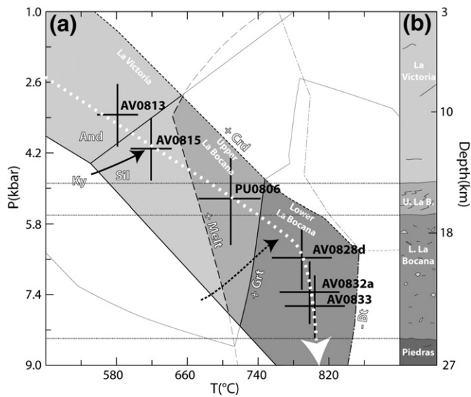
Fig. 12. P-T diagram for El Oro metamorphic complex. (a) reported peak P-T max conditions of studied samples in the simplified pseudosection of AV-08-15 sample (Fig. 8). Fields in greyscale show the domain of stability of observed mineral paragenesis of the La Victoria, the Upper and Lower La Bocana units. Note that the sample AV-08-15 (Fig. 5c) indicates that the pre-anatectic thermal history is marked by the transition from andalusite to kyanite, suggesting burial of the La Victoria unit before the high-temperature event (black arrow). The white and dashed arrows represent the maximum P-T condition recorded in the rock. We suggest that these last P-T conditions could represent the geothermal gradient during Triassic times. (b) Schematic structural log of the El Oro from the La Victoria unit to the South to the Piedras unit to the North.
