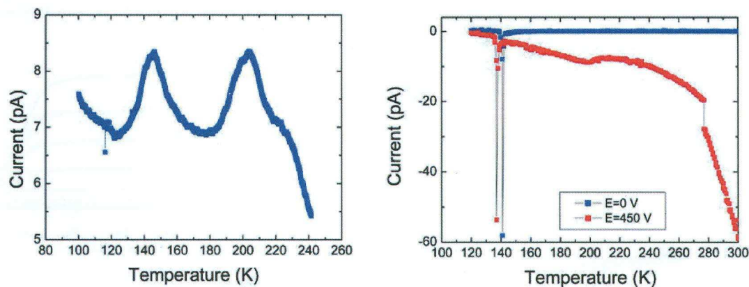
FIG. 6. (Color online) Discharge current anomalies in BiFeO 3 single crystals. (Left) pristine samples show two clear anomalies at \sim 140 and \sim 200 K, though in subsequent runs (right) only the 140 K anomaly is clear, although the 200 K anomaly is still visible for field-cooled samples. The field-cooling dependence of the peak temperature for the 140 K anomaly indicates that this pyroelectriclike current is due to the sudden carrier emission from trap levels triggered by the surface phase transition.
