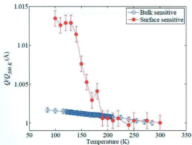
FIG. 4. (Color online) Relative change of the reciprocal lattice vector |g| as a function of temperature probing the bulk of a single crystal (blue open symbols) and the topmost surface (red solid symbols). The surface data show a rapid expansion of the lattice parameter upon heating above 140 K, and this feature is absent from the bulk.
