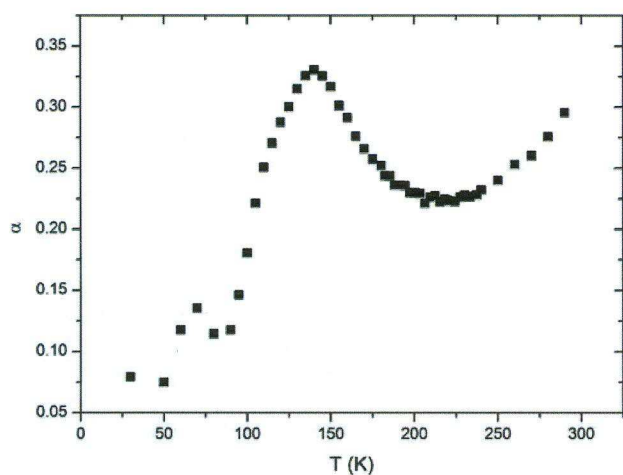
FIG. 7. Alpha parameter reflecting the asymmetry of the EPR curves for BFO nanotubes.
