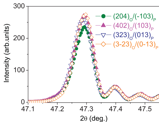
FIG. 3. (Color online) LaVO 3 XRD patterns recorded around the asymmetric diffraction peaks (204) o , (402) o , (323) o , and (3-23) o corresponding to the 103 p family. The matching between the intensities and the positions of the four peaks indicates that c_p is normal to the substrate plane.
