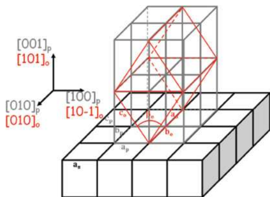
FIG. 4. (Color online) Schematic representation of the orientation of an epitaxial LaVO 3 thin film grown under compressive stress on a cubic (001)-oriented SrTiO 3 substrate. a_s is the substrate lattice parameter (3.905 Å); a_p , b_p , and c_p are the pseudocubic axes [ a_p = b_p = 3.91(3) Å, c_p = 3.945(1) Å] and a_o , b_o , and c_o are the orthorhombic axes; and \beta_o is the angle between a_o and c_o [ a_o = c_o = 5.55(2) Å, b_o = 7.82(6) Å, and \beta_o = 89.489(6)^\circ ].
