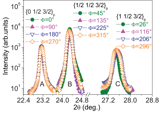
FIG. 7. (Color online) XRD patterns of equivalent half-order peaks. A, B, and C correspond to the peak family \{0 \frac{1}{2} \frac{3}{2}\}_p , \{\frac{1}{2} \frac{1}{2} \frac{3}{2}\}_p , and \{1 \frac{1}{2} \frac{3}{2}\}_p , respectively; see text for details.
